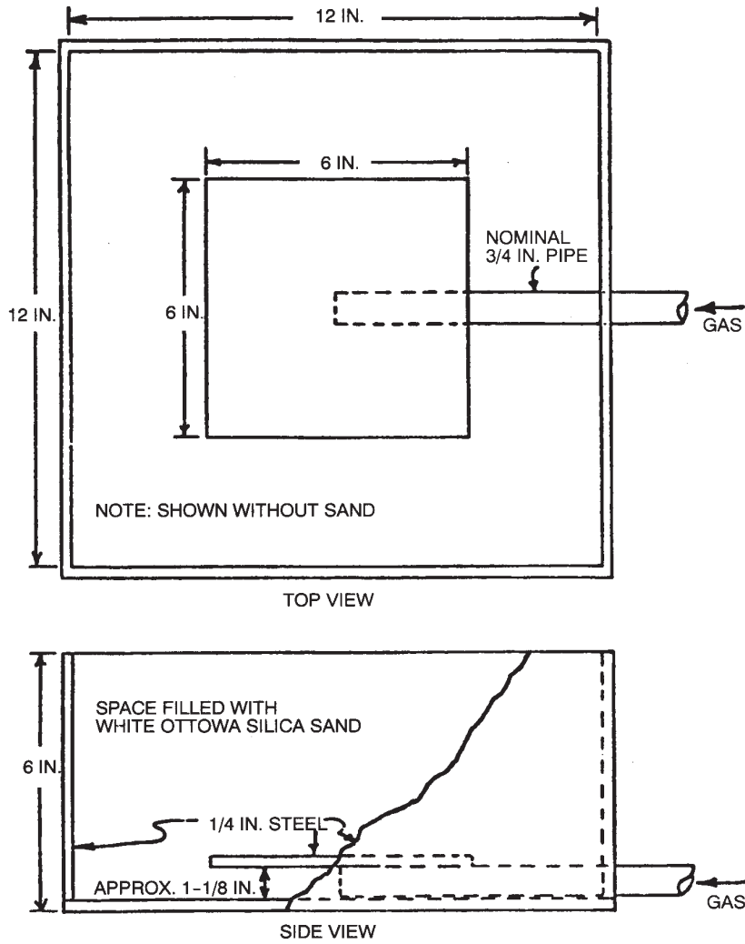
FIGURE 12-8-7—GAS BURNER
