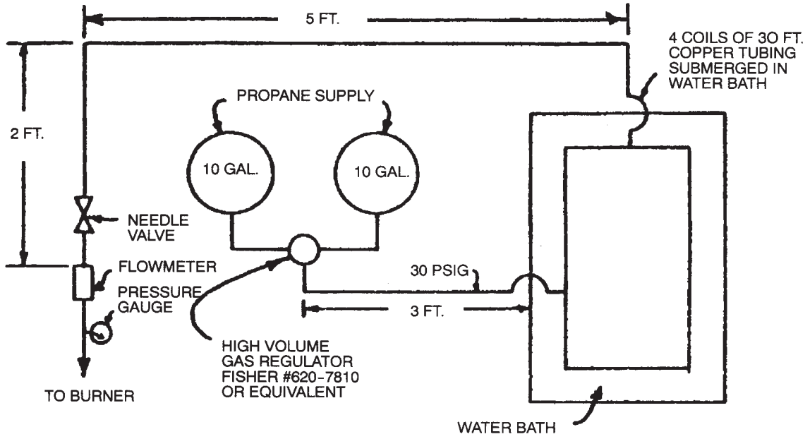
FIGURE 12-8-8—BURNER GAS FLOW CONTROL AND MEASUREMENT
