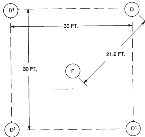
FIGURE 12-72-3-2—FIRE TEST DETECTOR INSTALLATION
