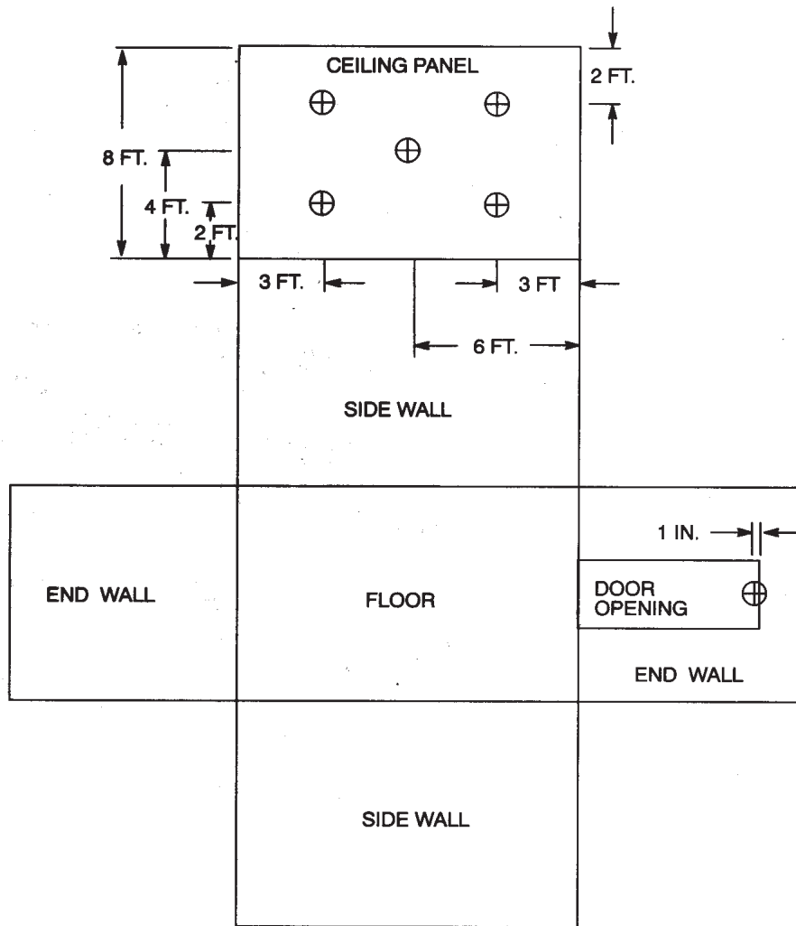
FIGURE 12-8-3—ROOM THERMOCOUPLE LOCATIONS
