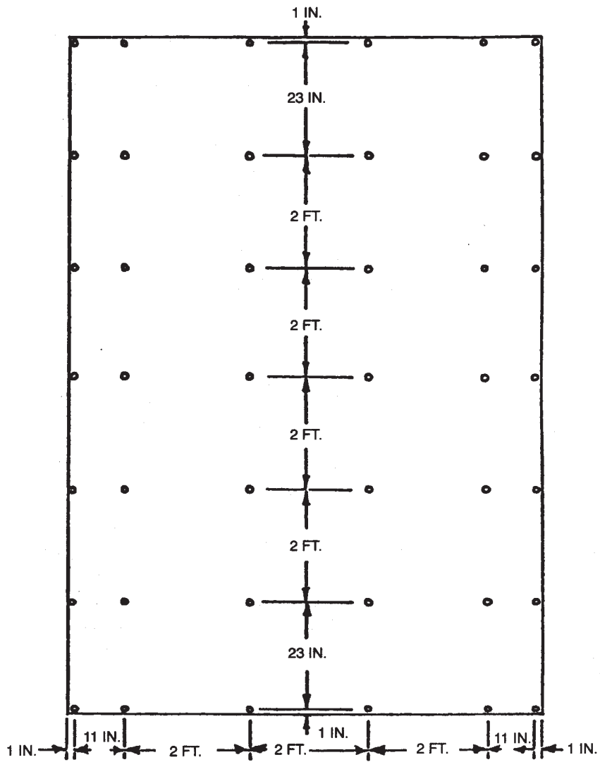
FIGURE 12-8-1B-5—TYPICAL MOUNTING TECHNIQUE FOR CEILING MATERIALS
