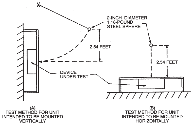
FIGURE 12-72-3-3—JARRING TEST
