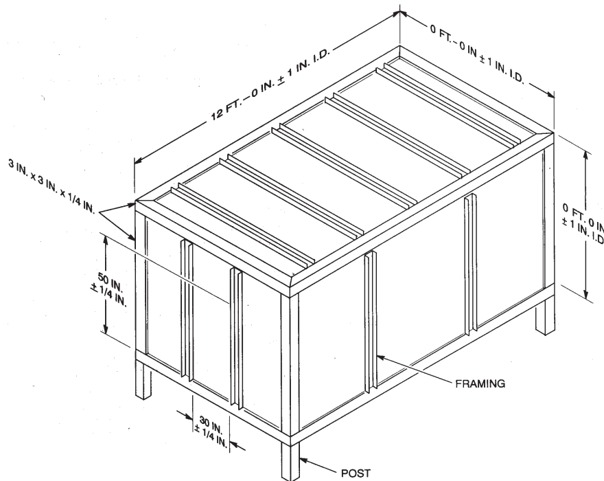
FIGURE 12-8-1B-1—TYPICAL STEEL FRAME SUPPORT SYSTEM
