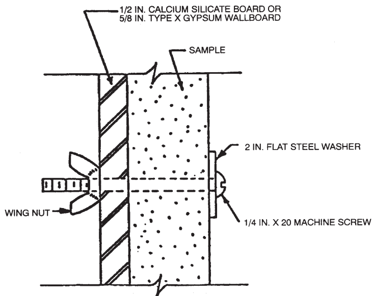
FIGURE 12-8-1B-2—MATERIAL FASTENING TECHNIQUE
