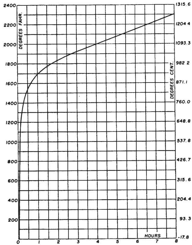
FIGURE 12-7-3-1—TIME-TEMPERATURE CURVE
