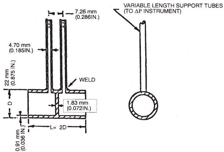
FIGURE 12-8-6—BIDIRECTIONAL PROBE
