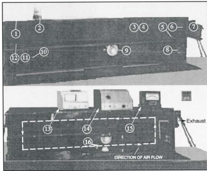
FIGURE 12-72-3-1—SMOKE DETECTOR TEST CHAMBER
