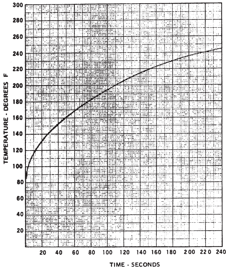
FIGURE 12-72-2-1—TIME-TEMPERATURE CURVE—15-FOOT SPACINGS
