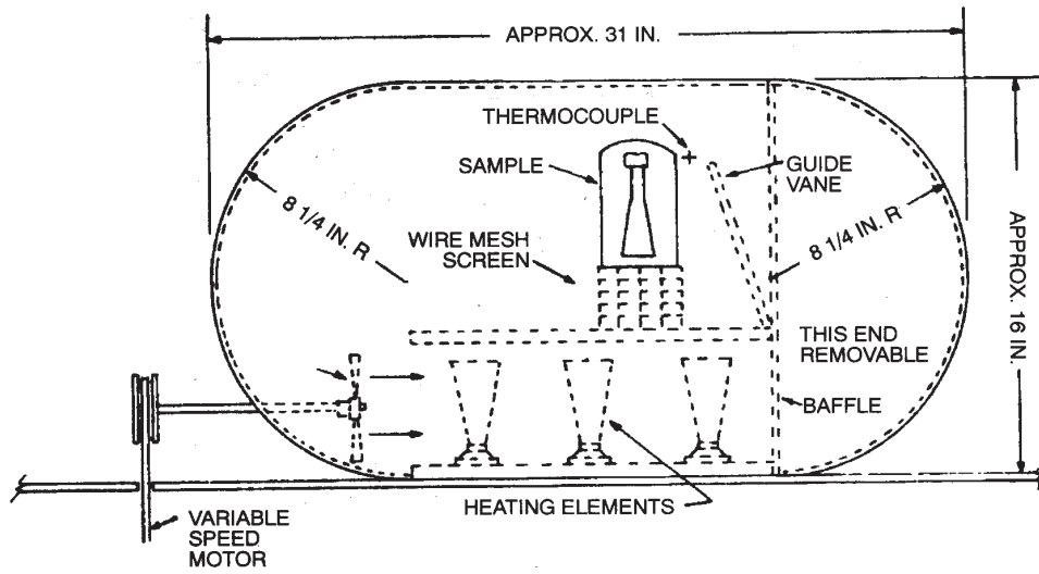
FIGURE 12-72-2-3—TEST OVEN
